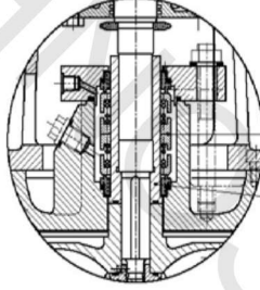
图三：叶轮名义直径<315mm,叶轮带副叶片，双端面机械密封。 Fig. 3 Impeller diameter<315mm, with back vanes, Double mechanical seal.
