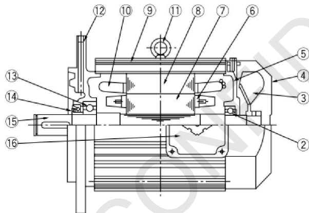
Fig.29 Example of construction of 80—112M frame
