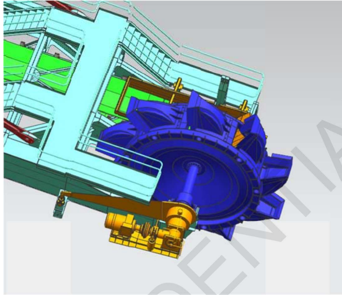
Figure 42. Bucket wheel Arrangement_(Plan View)
