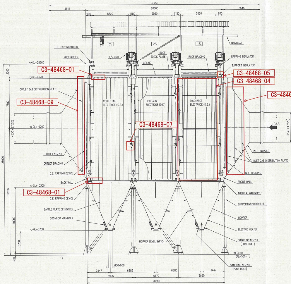
SECTION AA
