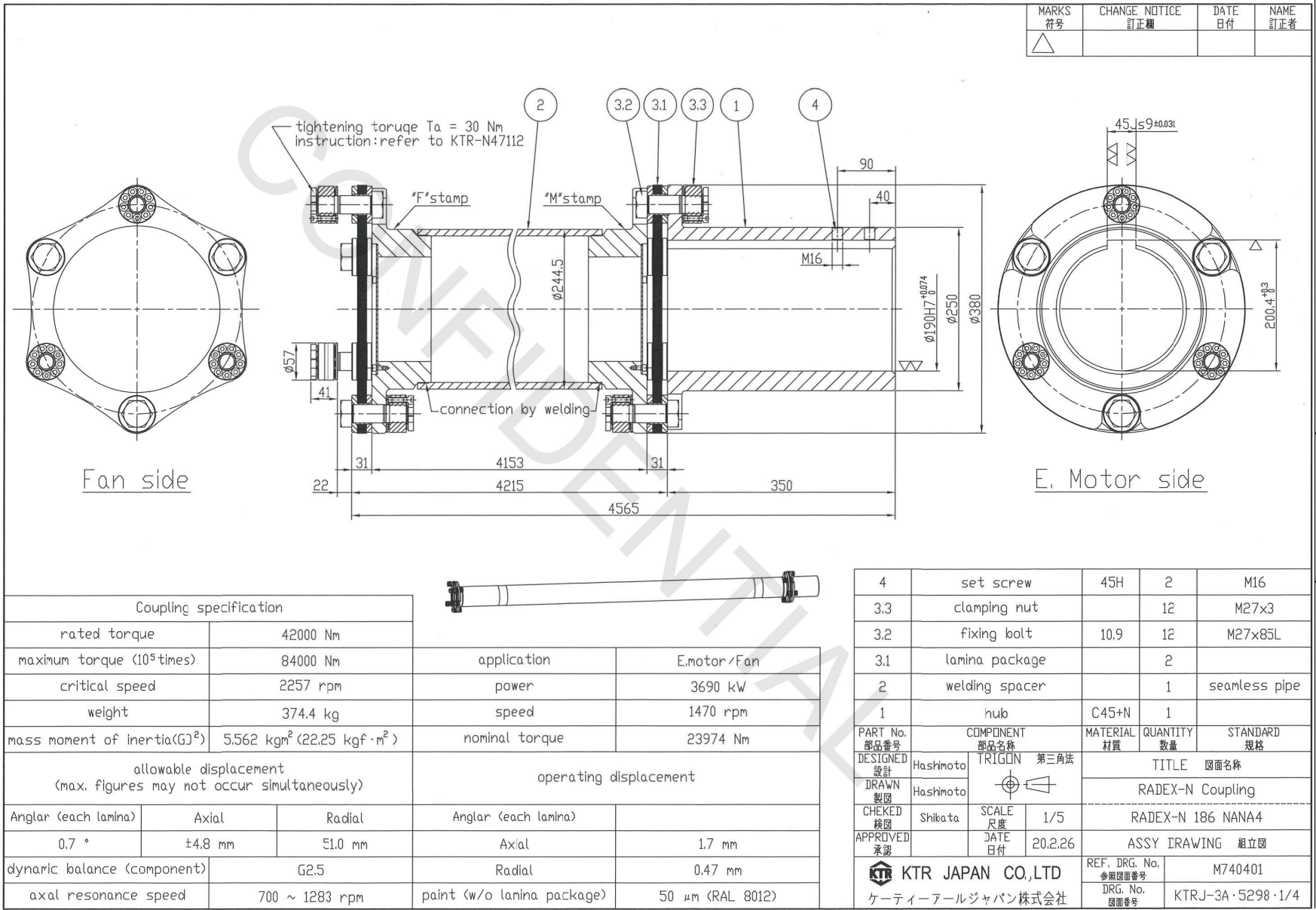
FIGURE 4-2.1.11 FLEXIBLE COUPLING FOR PA FAN
