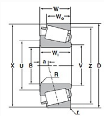
Tapered Roller Set - Inch Series and J Series - Dimensions
