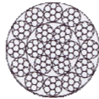
18x7 + WSC
