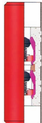
BUTT WELD FLOAT COLLAR WITH DOUBLE VALVE S-FCDV-BW-S101-12
