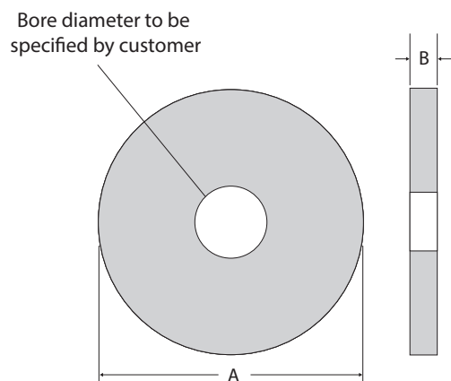
Figure 2: Plate Dimension Diagram for Universal Orifice Plates
