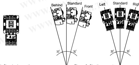
Figure 1 Standard mounting
