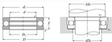
Single Direction Thrust Ball Bearings - Dimensions
