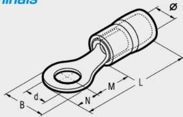
ring terminals
