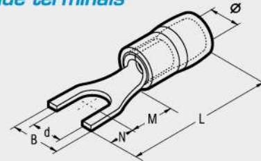
fork/spade terminals
