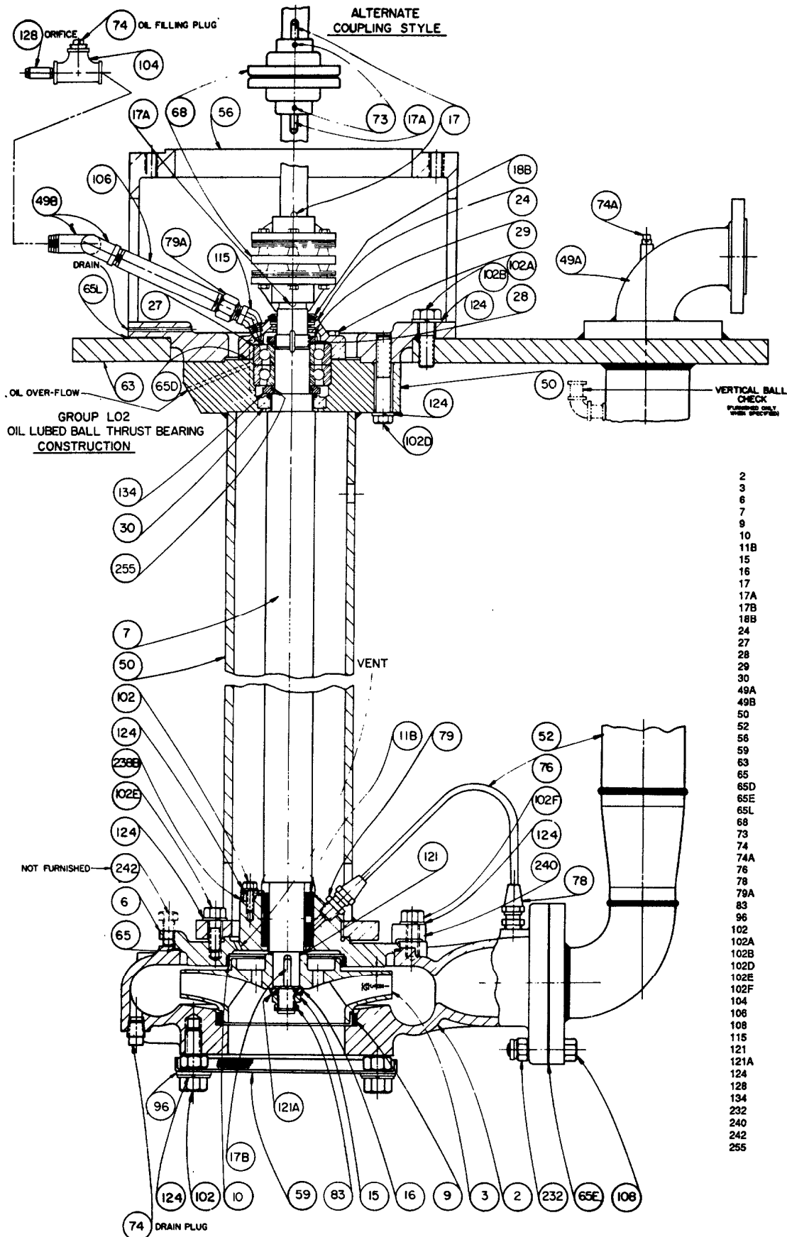
Figure 2. VCRE - VERTICAL LUBE OIL PUMP
